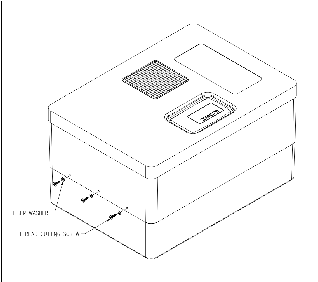
Figure 1. Installation Location of the Sealing Screws and Fiber Washers.
